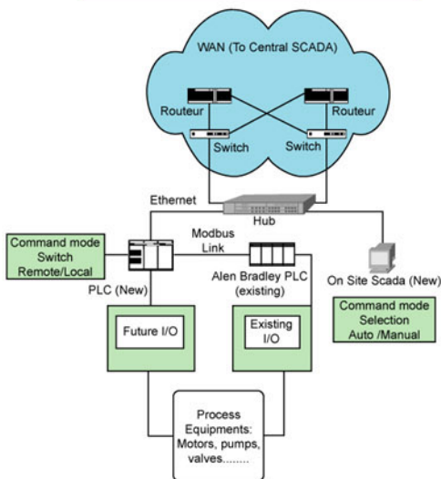
SIMPLIFIED STANDARD ARCHITECTURE FOR A PUMPING STATION (SINGLE NEW PLC)
